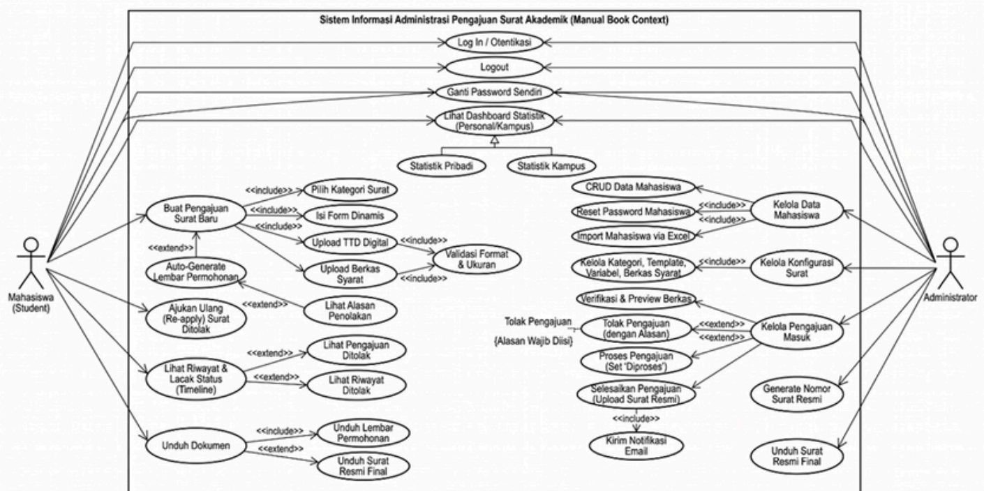
DIAGRAM USE CASE SISTEM ADMINISTRASI PENGAJUAN SURAT (TECHNICAL SCHEMATIC)
